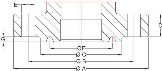
DIMENSIONS FOR CLASS 900, 1500 & 2500 RING TYPE JOINT
